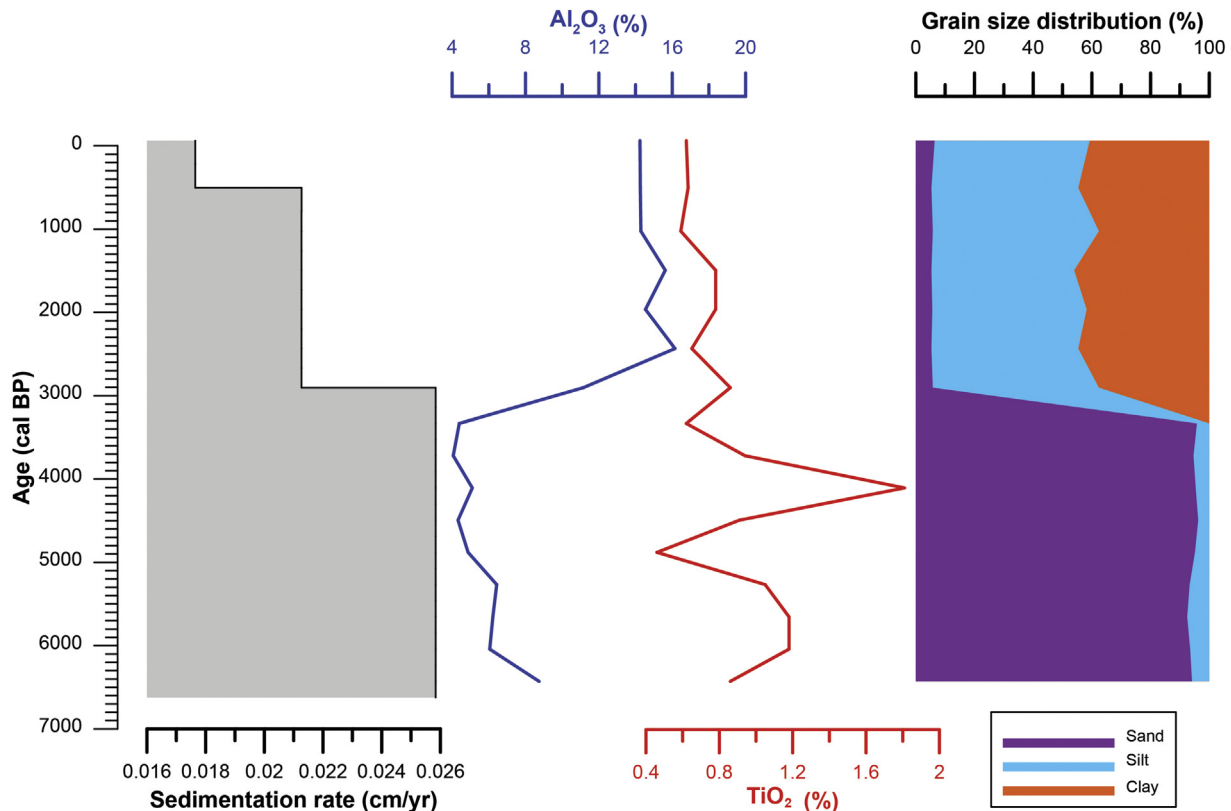
Fig. 4. The temporal variation in sedimentation rate, geochemical ( \text{Al}_2\text{O}_3 and \text{TiO}_2\% ), and grain size (sand, silt and clay %) data of core VC-04.
