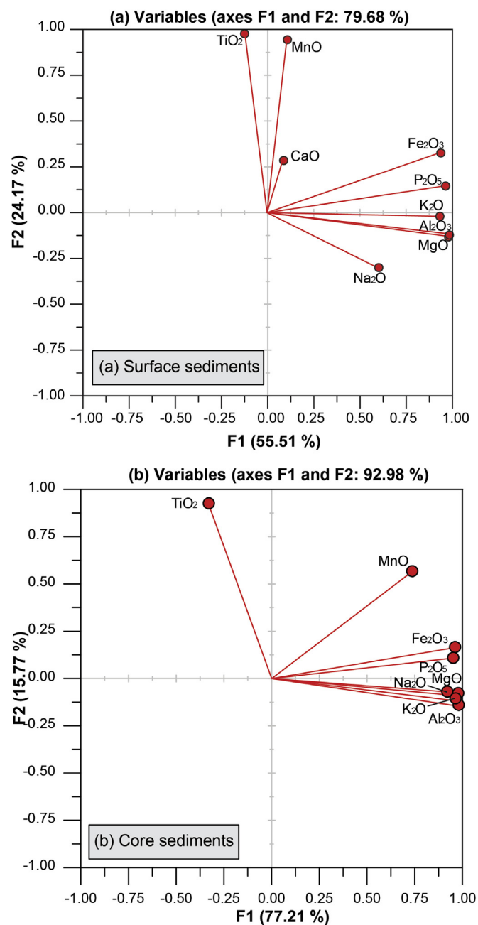
Fig. 2. Biplot of F1 axis vs. F2 axis based on the principal component analysis of geochemical parameters from (a) continental shelf surface sediments and (b) core sediments (VC-04).
