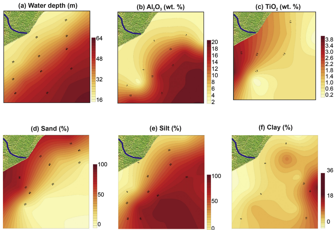
Fig. 3. a) Bathymetry of the study area, and spatial distribution of b) Al 2 O 3 (wt%), c) TiO 2 (wt%), d) Sand (%), e) Silt (%) and f) Clay (%) of the inner-mid continental shelf sediments adjacent to Rushikulya river mouth.
